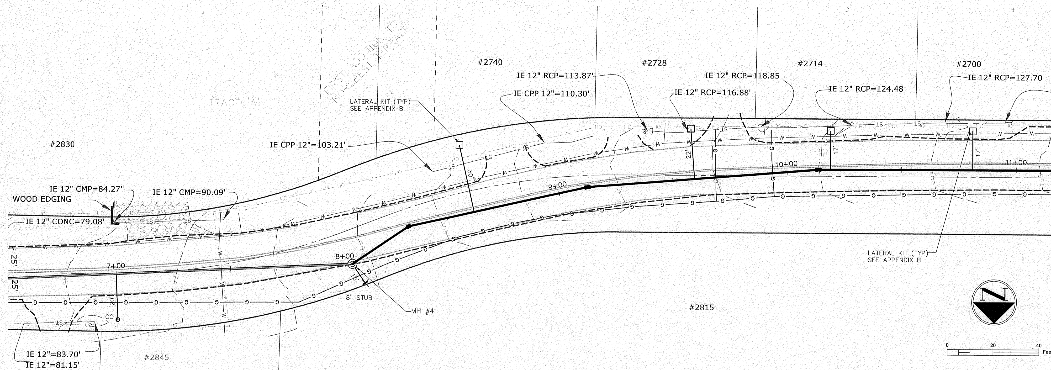
NE 36th Drive Plan View (STA 7+00 to 11+00)
