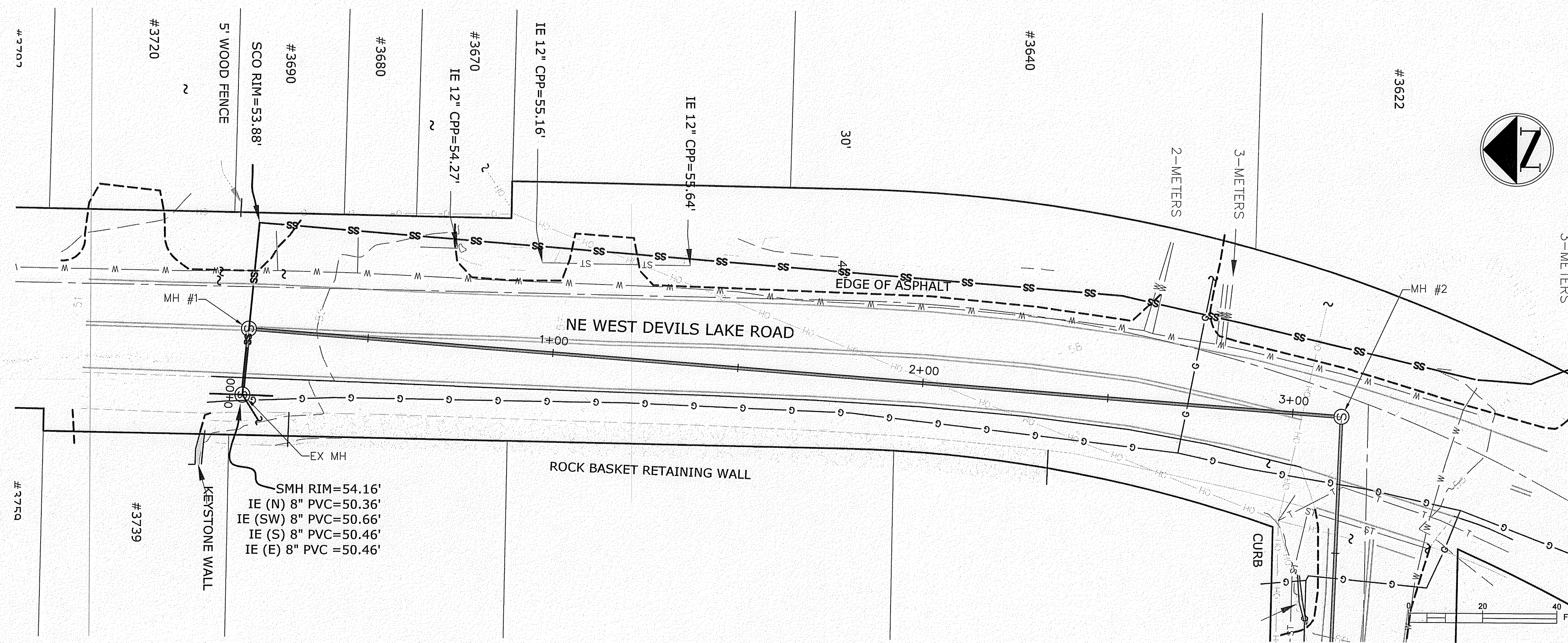
NE West Devils Lake Rd. Plan View
