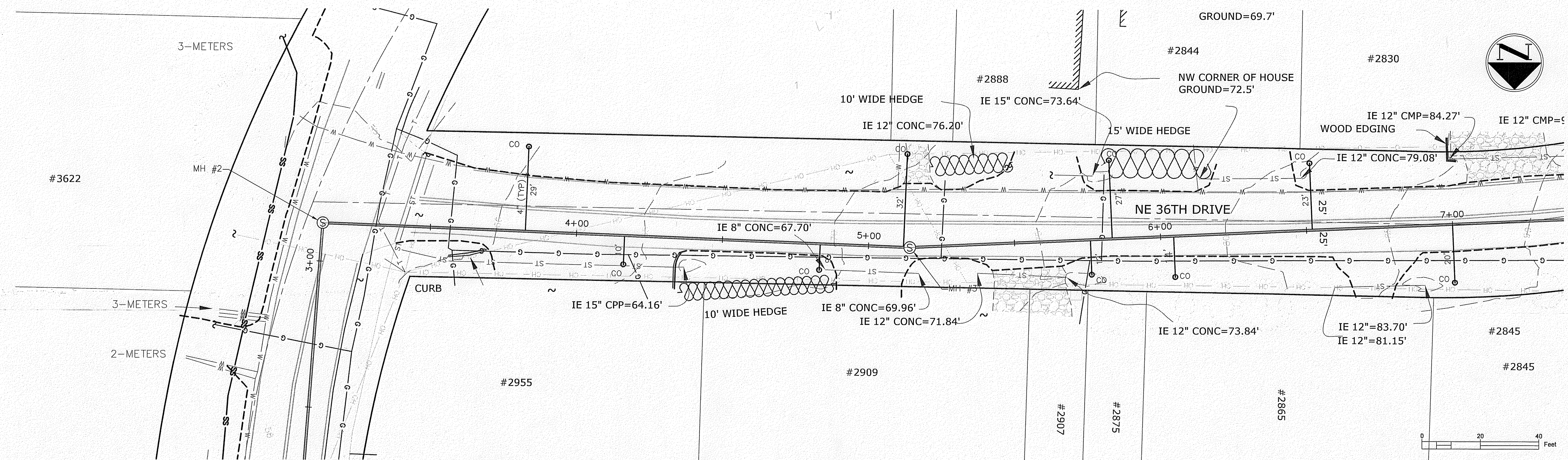
NE 36th Drive Plan View (STA 3+00 to 7+00)
