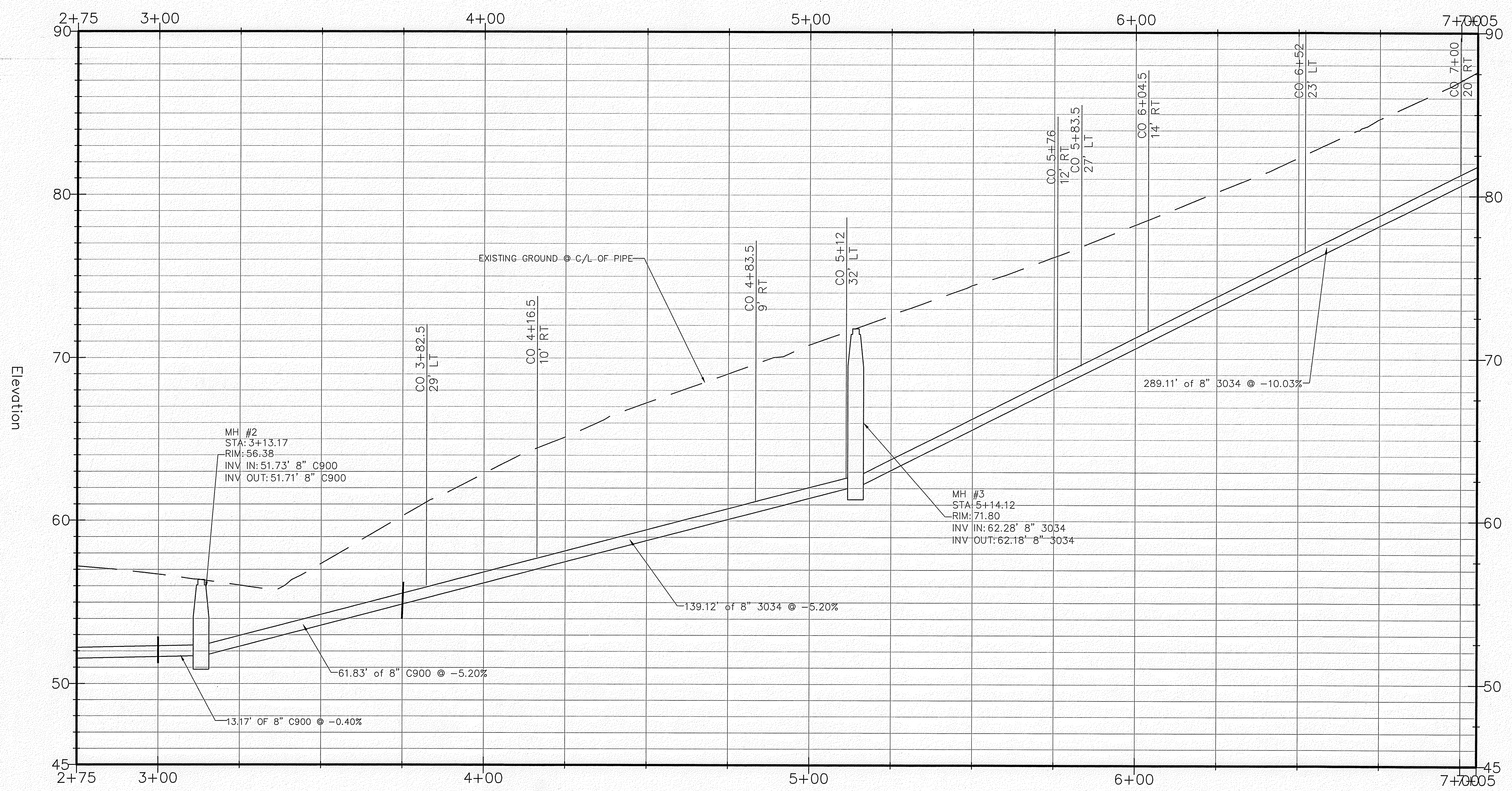
NE 36th Drive Sanitary Sewer Profile (STA 3+00 to 7+00)
