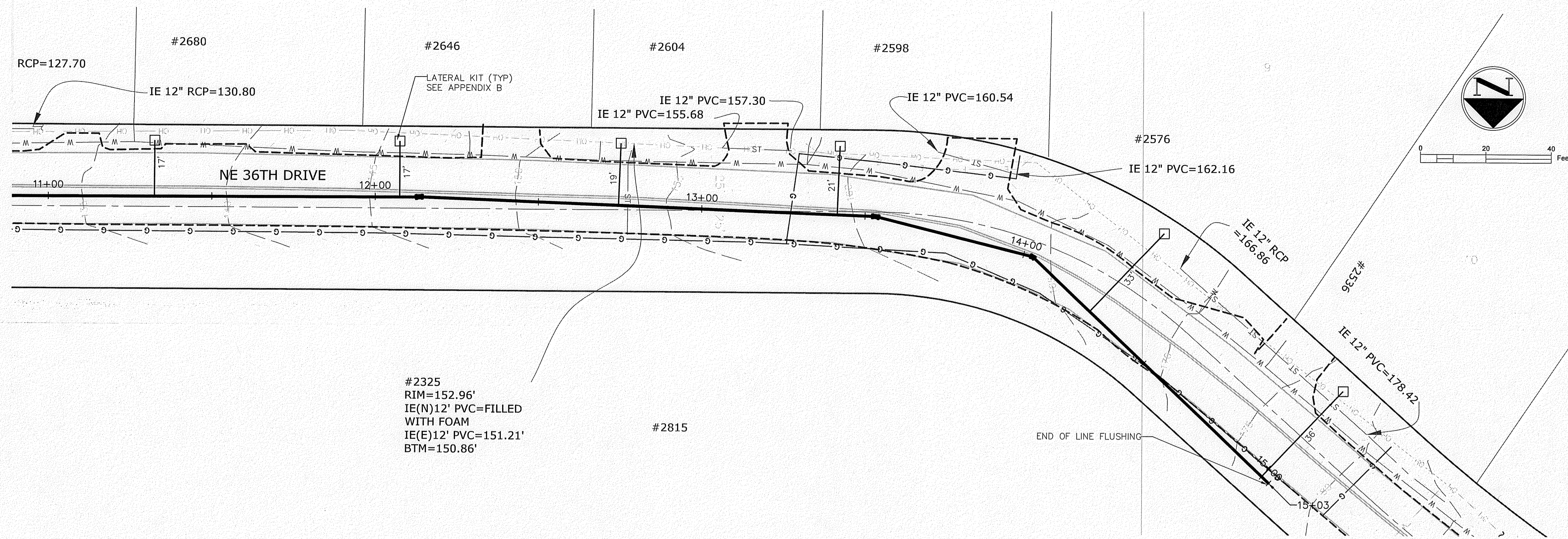
NE 36th Drive Plan View (STA 11+00 to 15+00)
