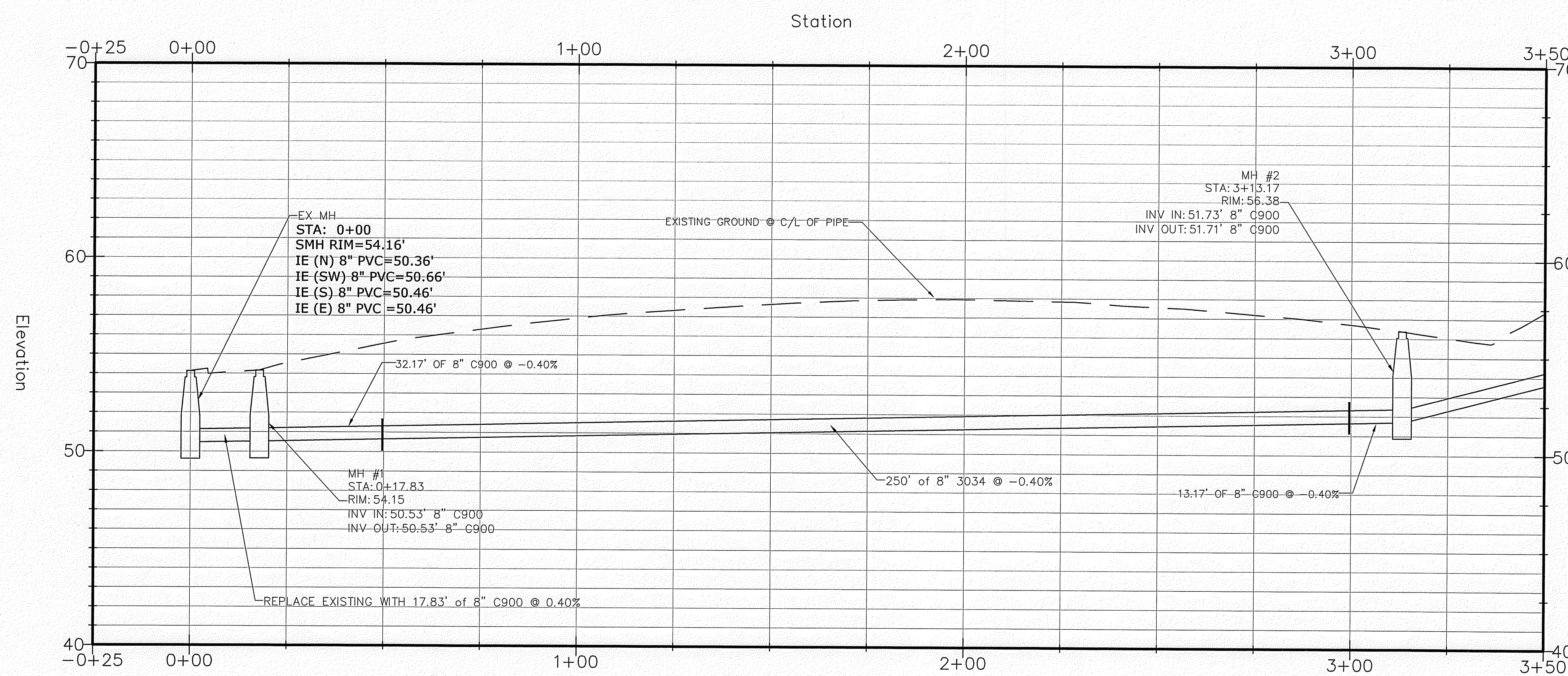
NE West Devils Lake Rd. Sanitary Sewer Profile (STA 0+00 to 3+50)
